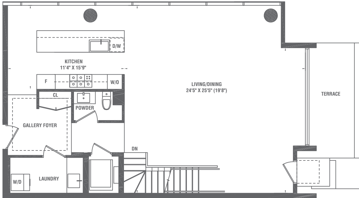
GROUND FLOOR
