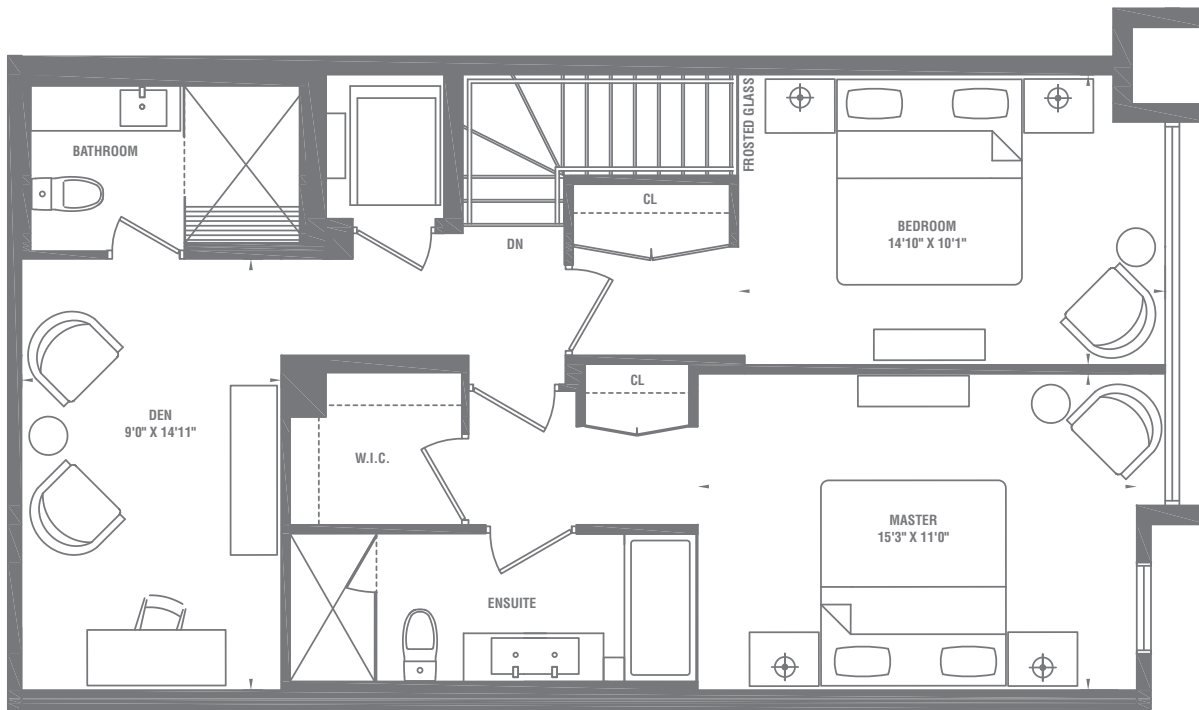
SECOND FLOOR
